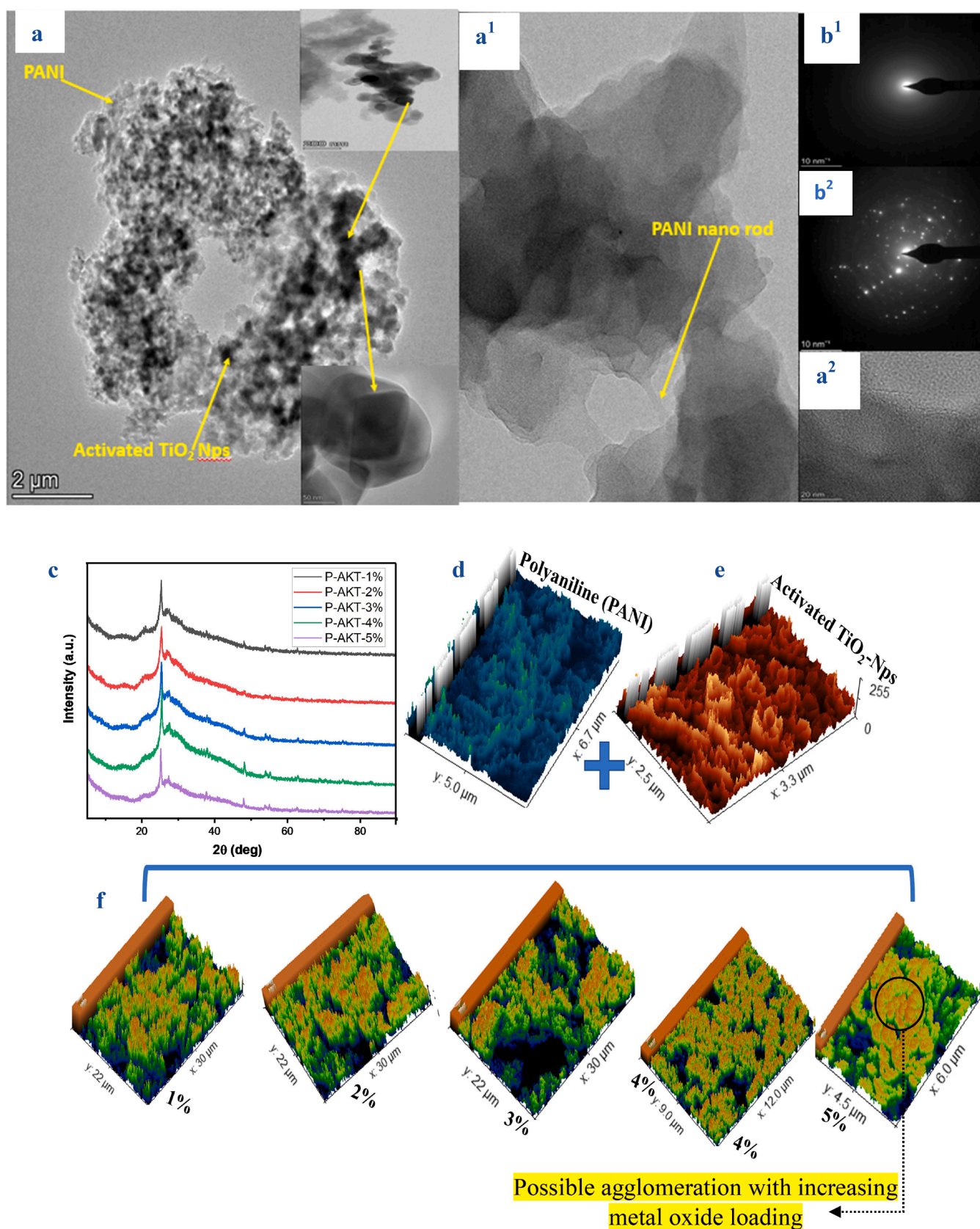
Fig. 3. (a-a 2 ) HR-TEM of P-AKT-3 % (b) SAED pattern for P-AKT-3 % (c) XRD pattern of P-AKT-1 to 5 % (d) 3D surface imaging of PANI and (e) Activated TiO 2 Nps; (f) Composites P-AKT-1 %; 2 %; 3 %; 4 %; 5 %.
