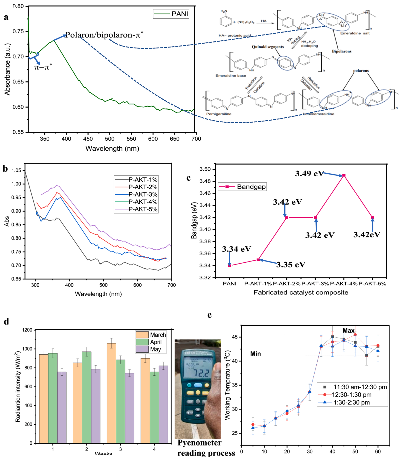
Fig. 6. (a) UV-vis analysis of PANI and (b) P-AKT-1 % to 5 %; (c) bandgap result of photocatalyst; (d) Measurement of solar radiation (e) measurement of working temperature.
