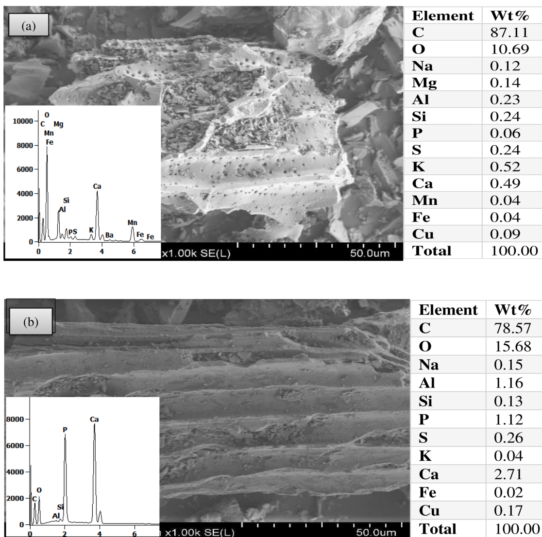
Fig. 2. The SEM micrograph and EDX spectra for (a) seaweed biochar (SB) and (b) Hydroxyapatite activated biochar (HSB) at 50.0 μm.
