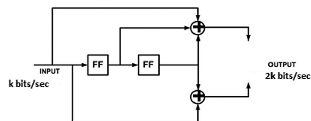
Figure 3. Convolutional encoder.
