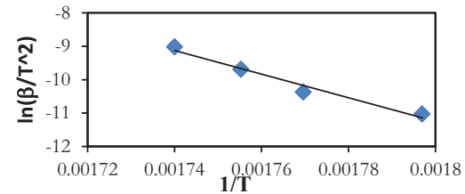
Figure 5: Determination of kinetic parameter of Arusha municipal solid waste.
