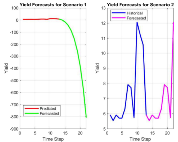
Fig. 5. The plot of banana crop yield forecasting for the State Space model.
