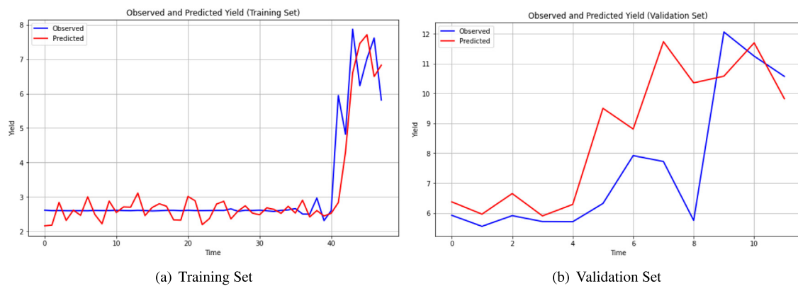
Fig. 2. The observed and predicted banana crop yield for the SARIMAX model.
