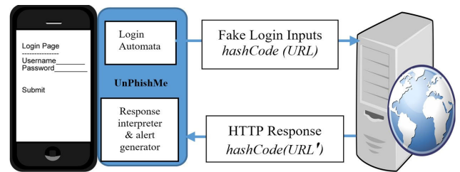
FIGURE 7. Checking HTTP response and URL consistency.
