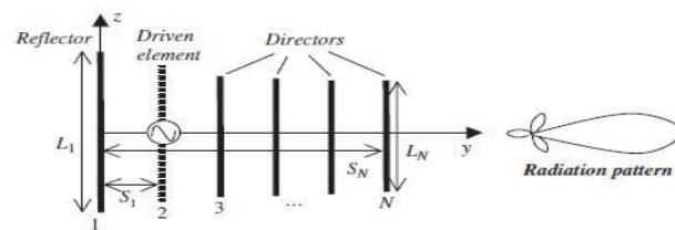
Figure 4: Source: Yagi Uda antenna structure Huang and Boyle (2008)
