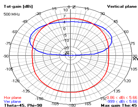
Figure 5: Radiation pattern before optimization
