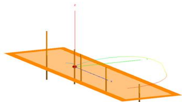
Figure 10: Optimized Yagi-Uda Antenna
