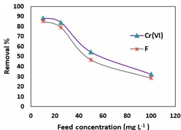
Figure 1 | Comparison of the electrosorption capacity of F^- and Cr(VI) . Reprinted from (Gaikwad & Balomajumder 2017b), copyright (2017), with permission from Elsevier.
