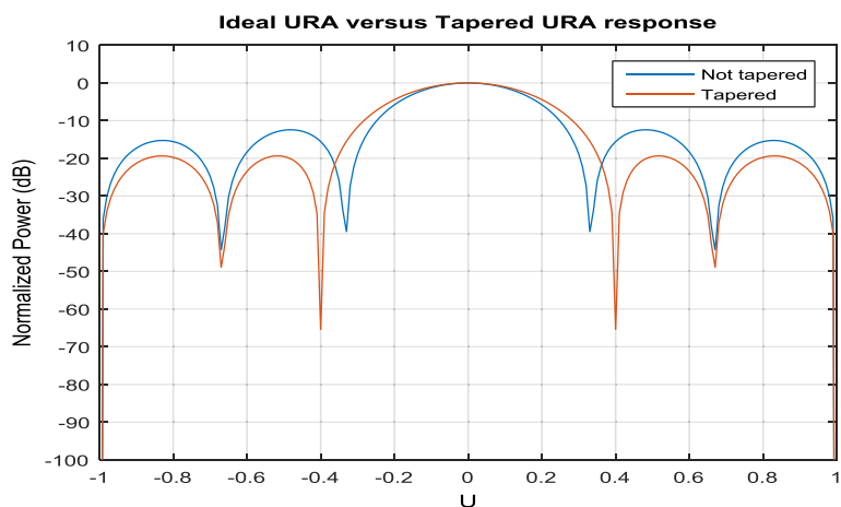
Figure 15. Tapering response.
