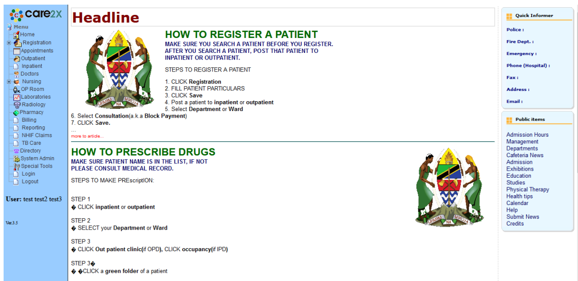
Figure 4: Care2x dashboard
