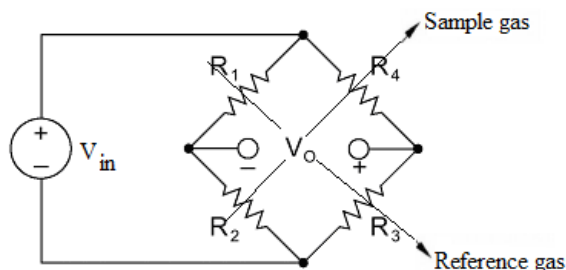
Figure 4: Wheatstone bridge configuration
