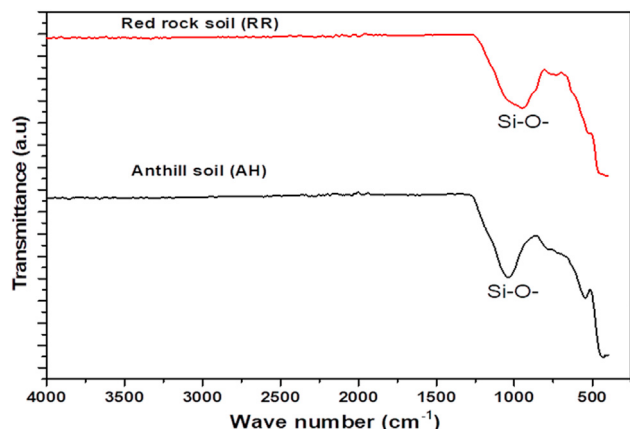
Fig. 2. FTIR spectra of AH and RR.
