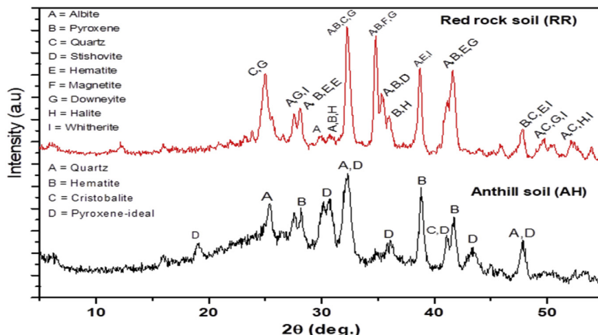
Fig. 1. XRD spectra of anthill (AH) and red rock (RR) soil samples.
