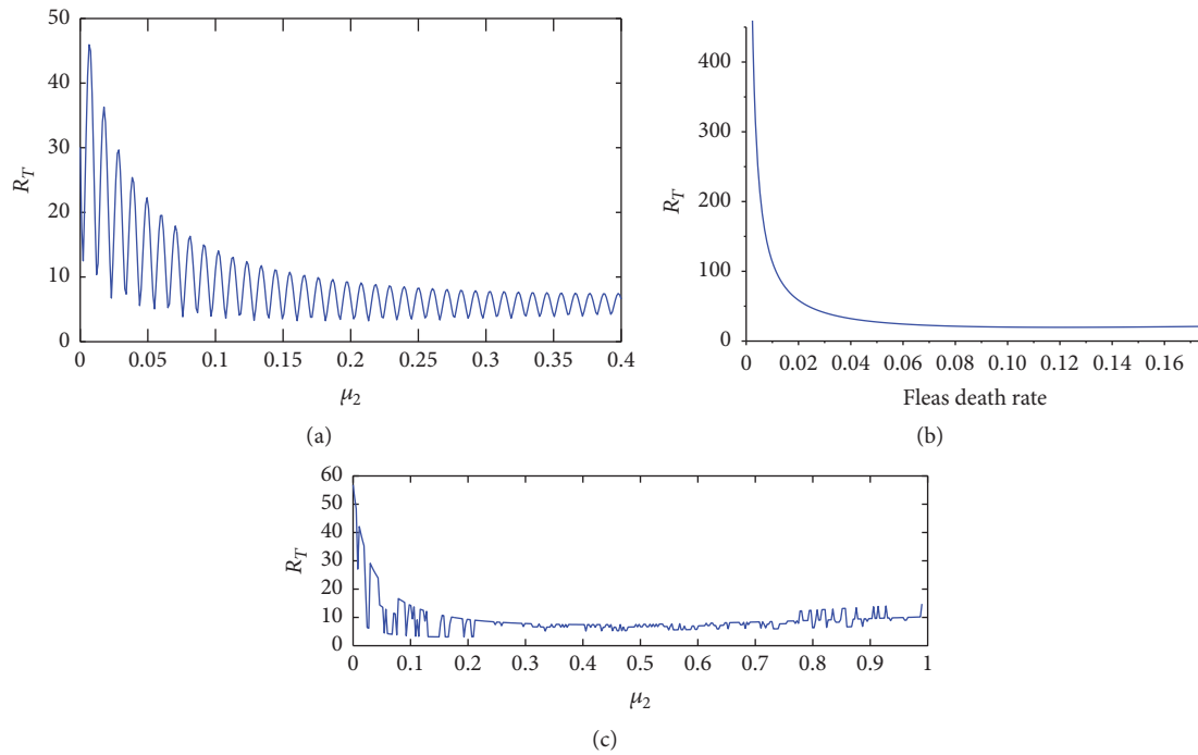
FIGURE 7: Effect of increased number of fleas' death rate on the periodic reproduction number.
