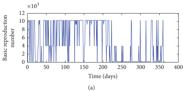
FIGURE 16: Distribution of R_0 based on fluctuation of temperature (a) and relative humidity (b) data in Mtwarea.
