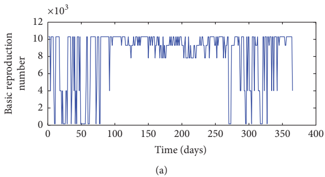
FIGURE 18: Distribution of R_0 based on fluctuation of temperature (a) and relative humidity (b) data in Tanga.
