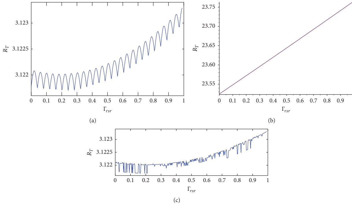
FIGURE 13: Effect of infection rate ( \Gamma_{rsr} ) on the periodic reproduction number.
