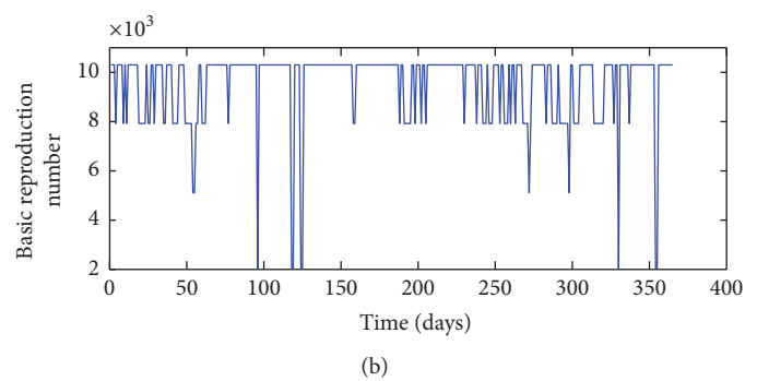
FIGURE 18: Distribution of R_0 based on fluctuation of temperature (a) and relative humidity (b) data in Tanga.
