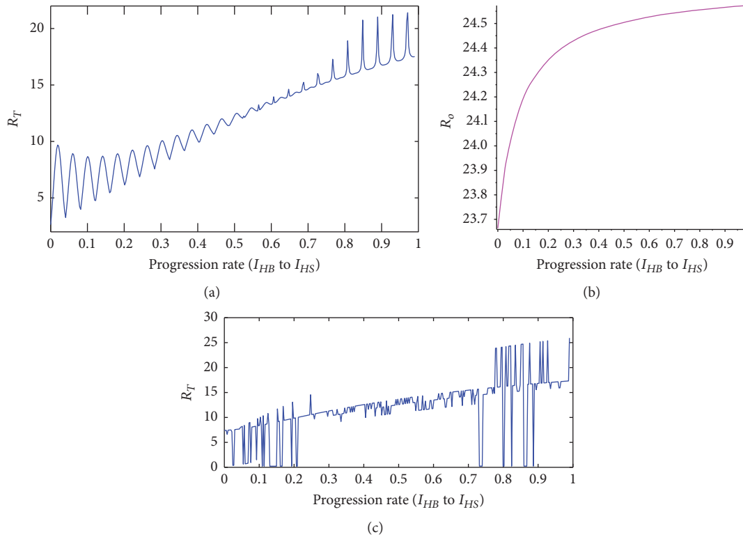
FIGURE 1: Effect of progression rates from I_{HB} to I_{HS} on the periodic reproduction number.
