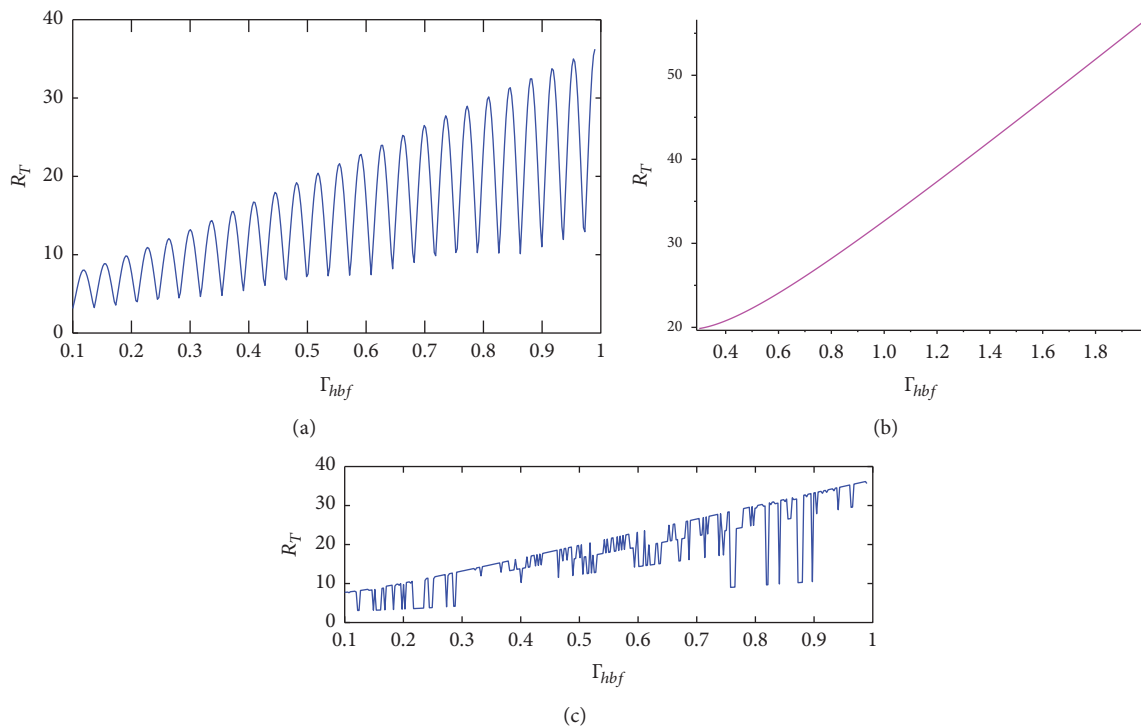
FIGURE 8: The effect of increased infection rate to fleas from the infectious human beings ( I_{HB} ) on the periodic reproduction number.
