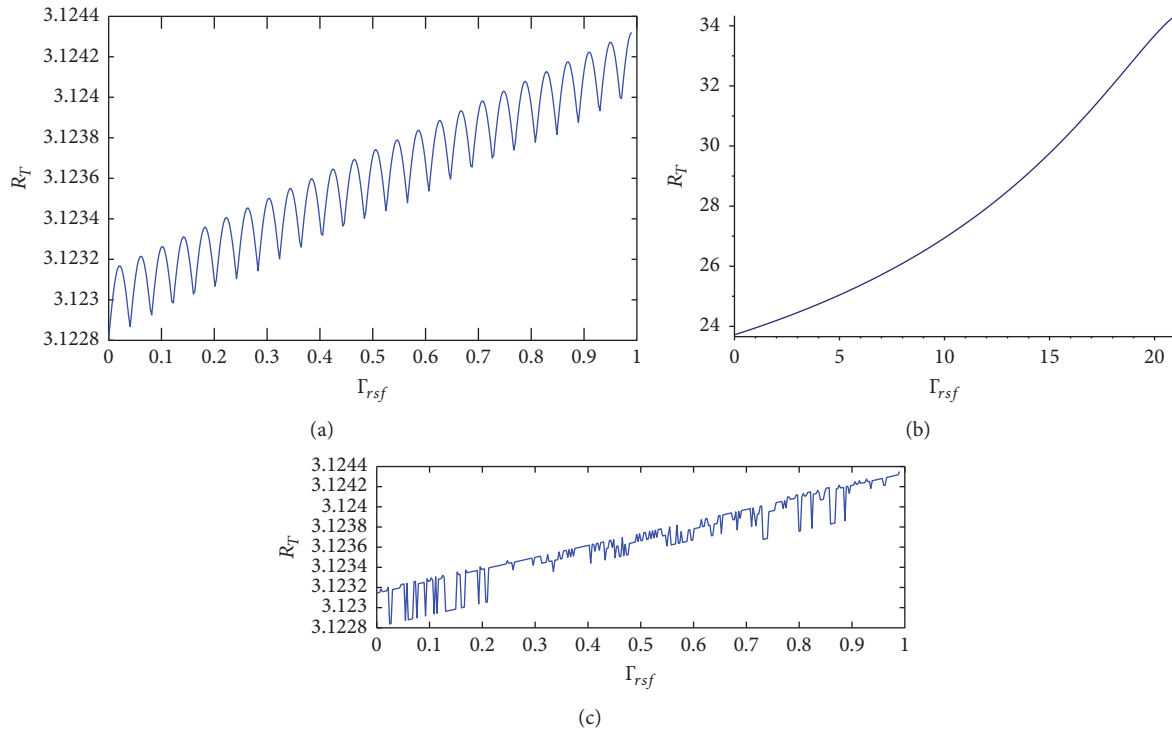
FIGURE 11: The effect of increased infection rate to fleas from the infectious rodents ( I_{RS} ) on the periodic reproduction number.
