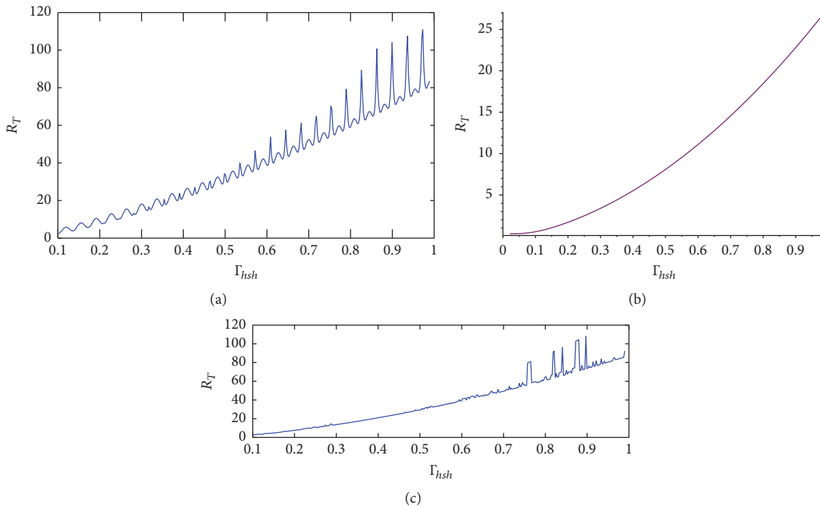
FIGURE 12: Effect of infection rate ( \Gamma_{hsh} ) on the periodic reproduction number.
