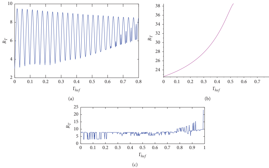
FIGURE 9: The effect of increased infection rate to fleas from the infectious human beings ( I_{HS} ) on the periodic reproduction number.
