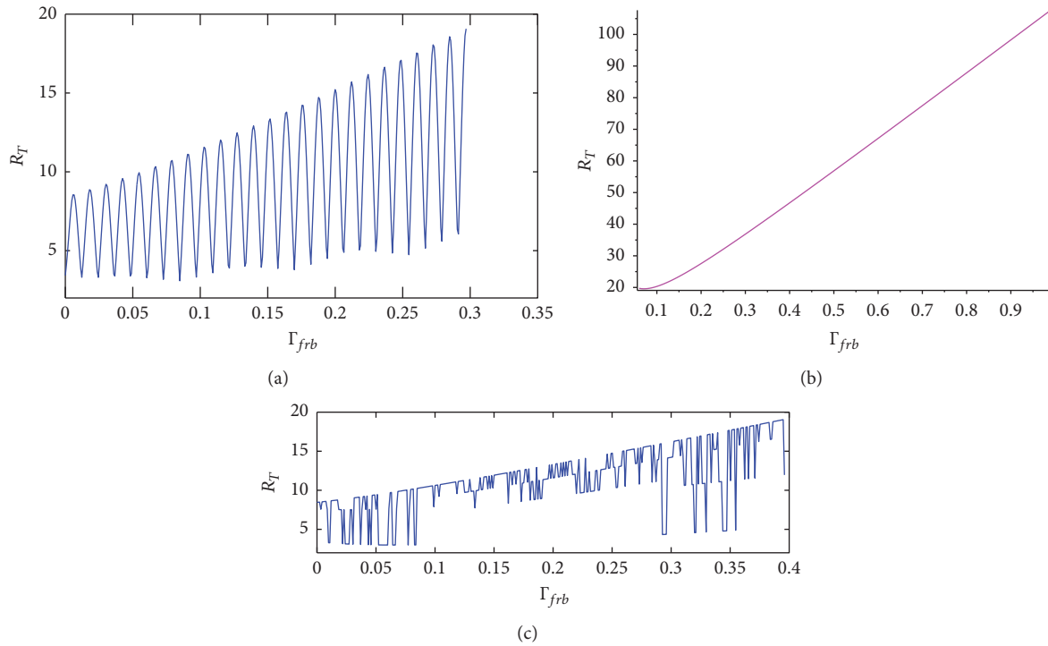
FIGURE 5: The effect of infection from I_F to rodents with bubonic plague on the periodic reproduction number.
