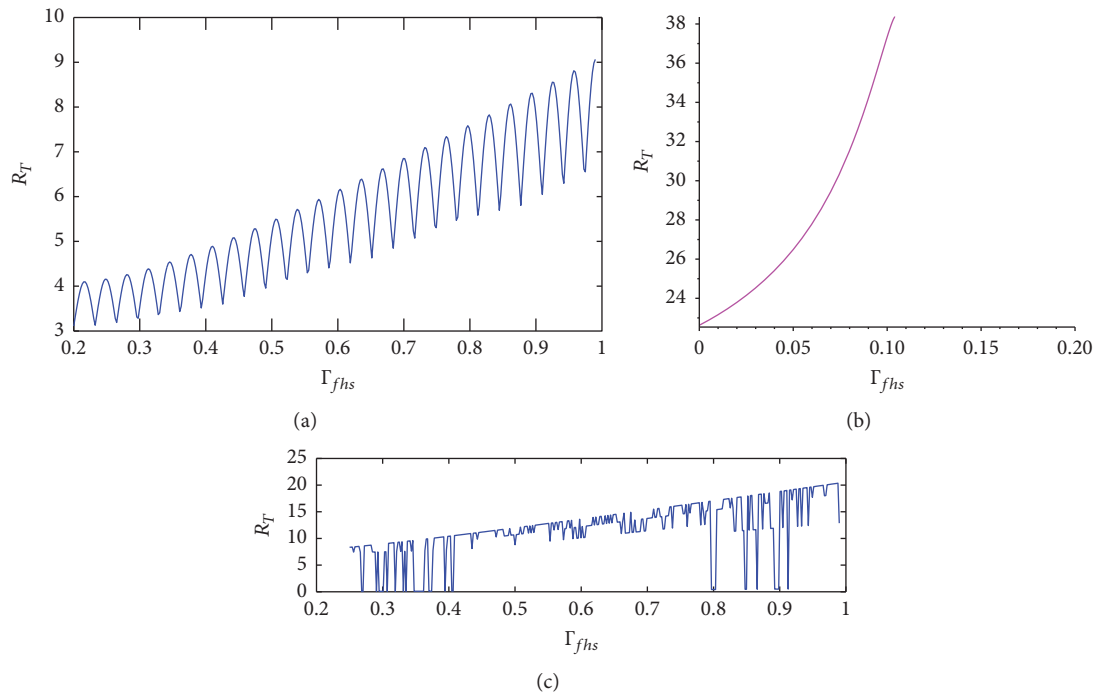
FIGURE 4: The effect of infection from I_F to human beings with septicemic plague on the periodic reproduction number.
