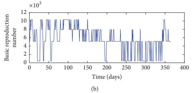
FIGURE 17: Distribution of R_0 based on fluctuation of temperature (a) and relative humidity (b) data in Singida.
