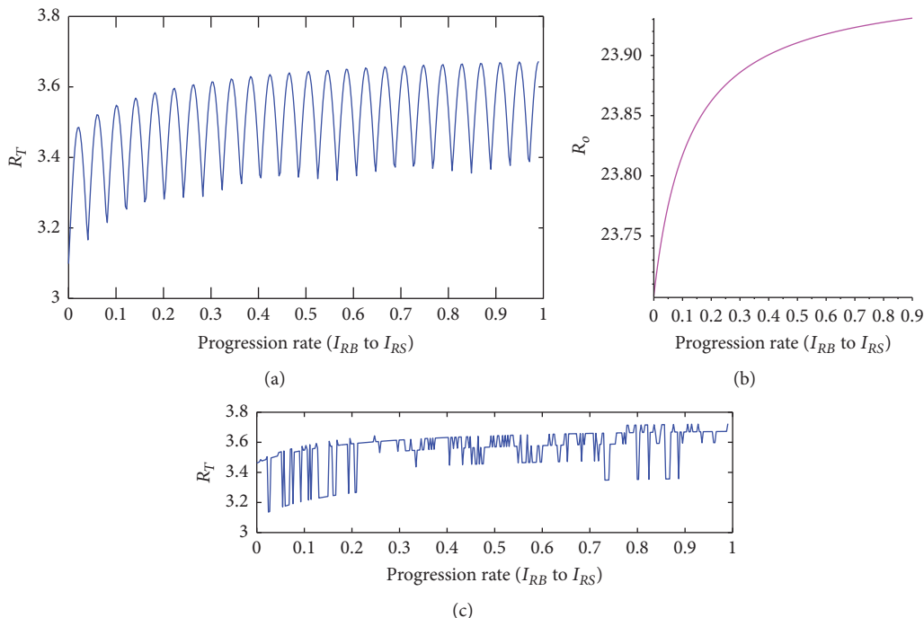
FIGURE 2: Effect of progression rates from I_{RB} to I_{RS} on the periodic reproduction number.
