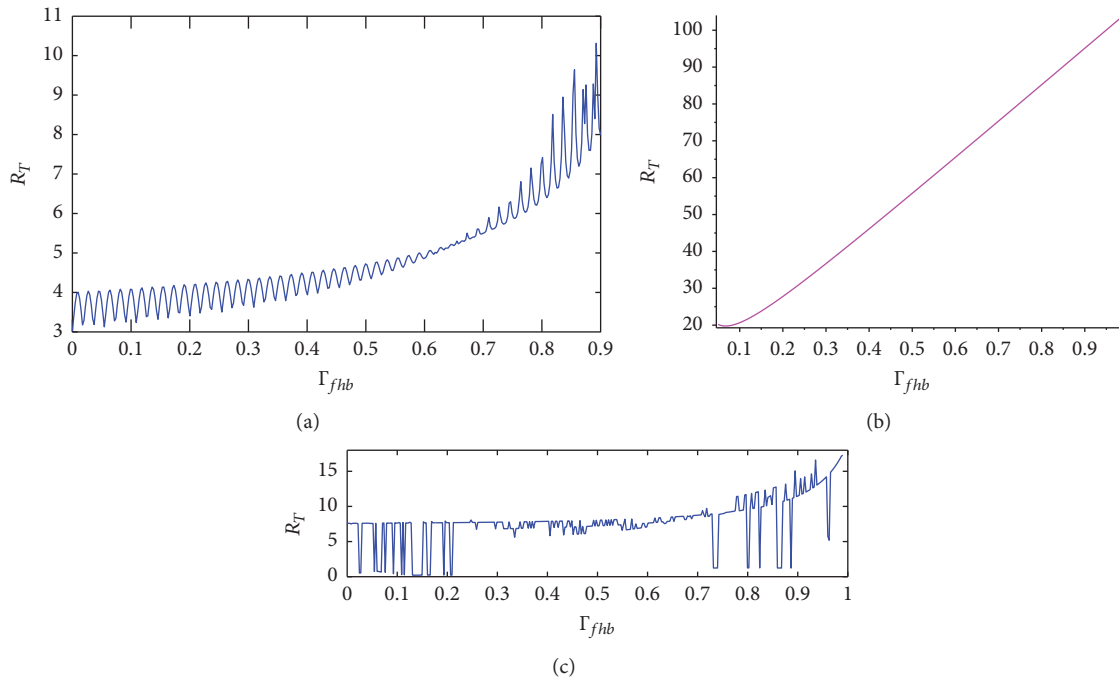
FIGURE 3: The effect of infection from I_F to human beings with bubonic plague on the periodic reproduction number.
