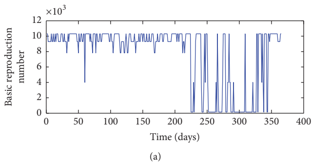
FIGURE 15: Distribution of R_0 based on fluctuation of temperature (a) and relative humidity (b) data in Mbeya.
