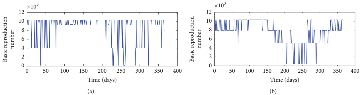
FIGURE 14: Distribution of R_0 based on fluctuation of temperature (a) and relative humidity (b) data in Kigoma.
