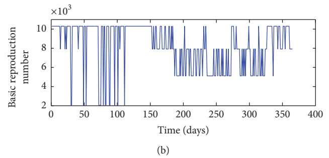
FIGURE 16: Distribution of R_0 based on fluctuation of temperature (a) and relative humidity (b) data in Mtwarea.
