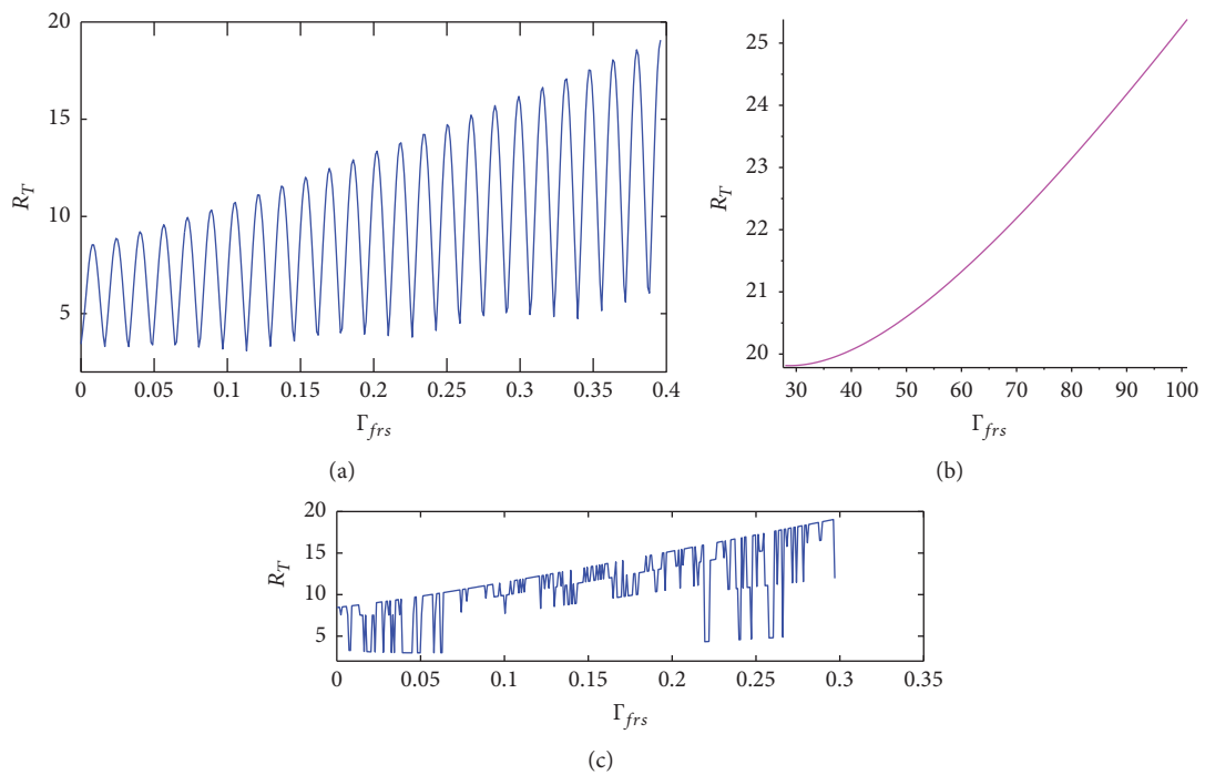
FIGURE 6: The effect of infection from I_F to rodents with septicemic plague on the periodic reproduction number.
