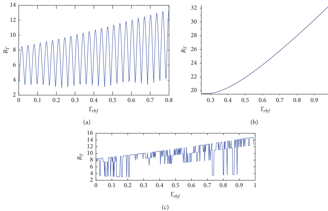
FIGURE 10: The effect of increased infection rate to fleas from the infectious rodents ( I_{RB} ) on the periodic reproduction number.
