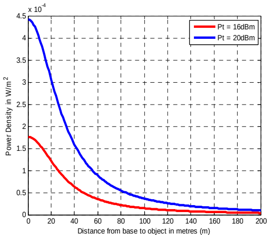
Figure 2: Power density versus distance of a point for P_t = 16 dBm, 20dBm and a gain G_t = 17 dB
