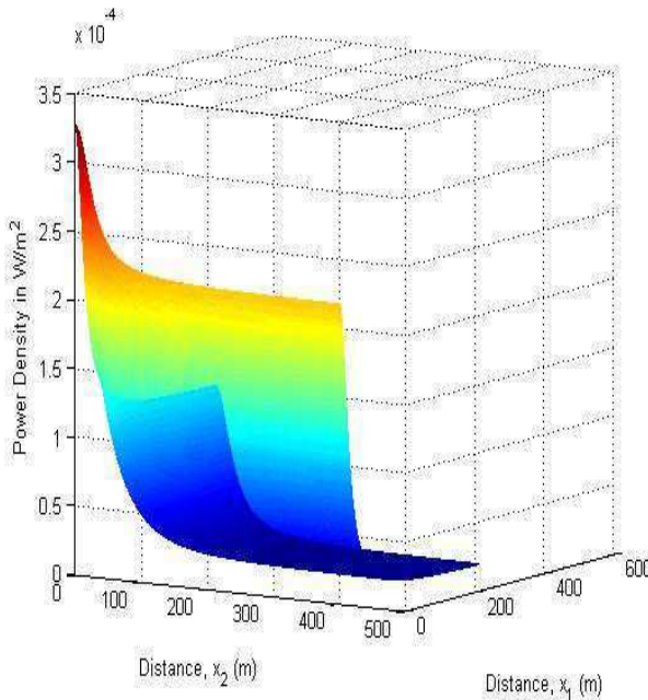
Figure 7: Power Density from two towers for an object at a height h_0=3m
