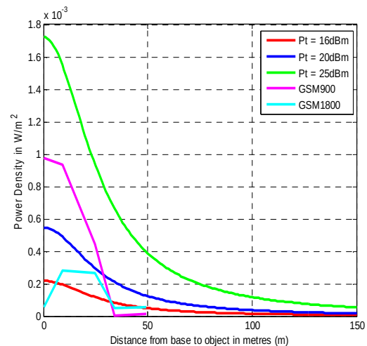
Figure 3: Power Density with fixed height of object h_0 = 3 m in various P_t
