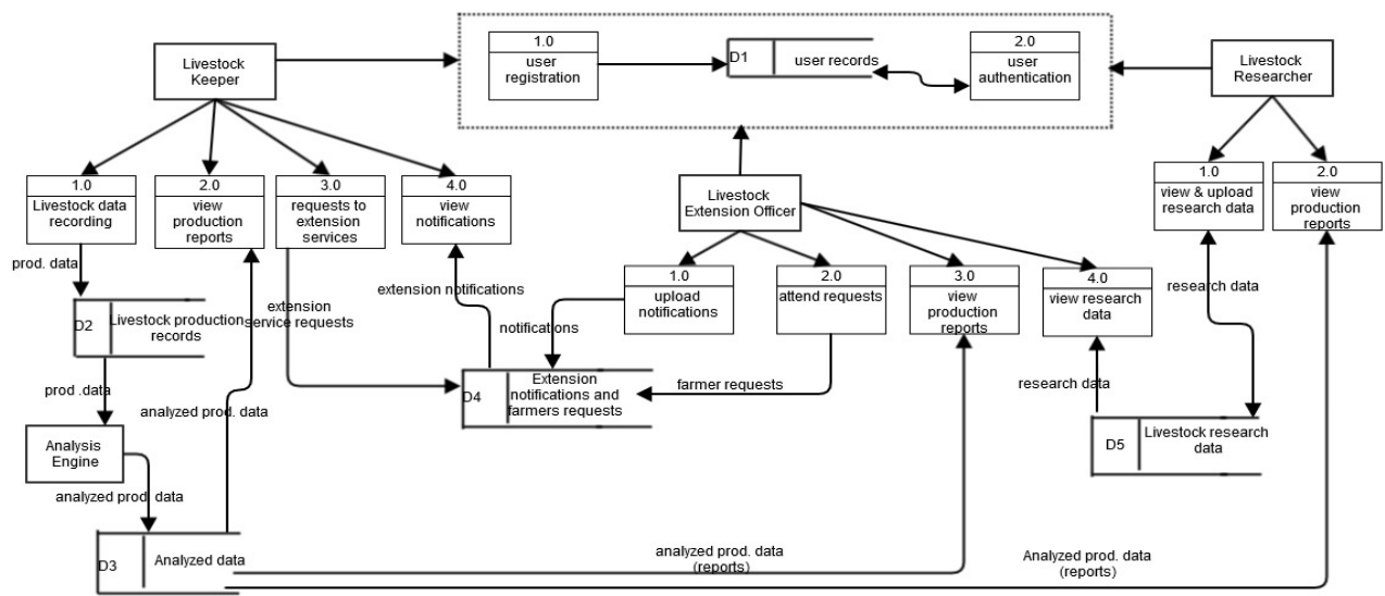
Figure 3. DFD level 1
