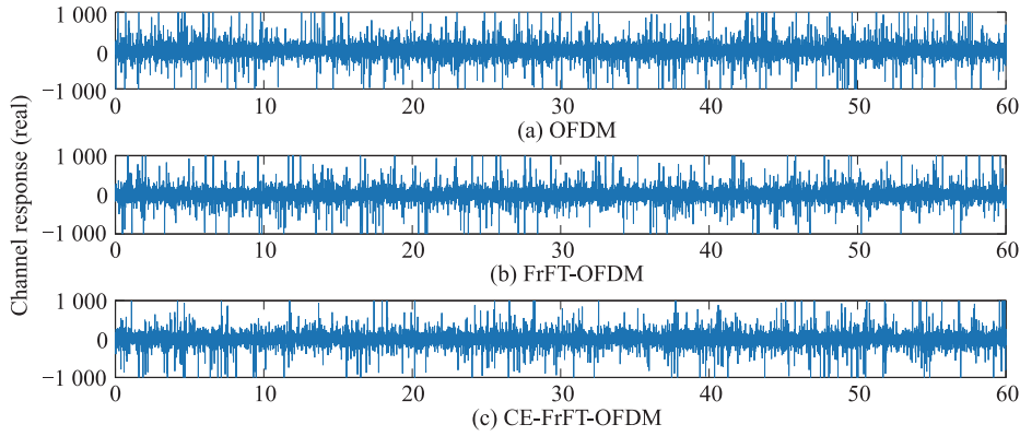
Fig. 2 OFDM, FrFT-OFDM, and CE-FrFT-OFDM channel impulse responses
