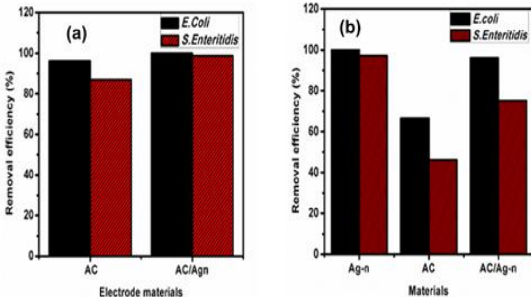
Figure 15: Bacteria removal efficiency (a) during the CDI process (b) by physical contact.
