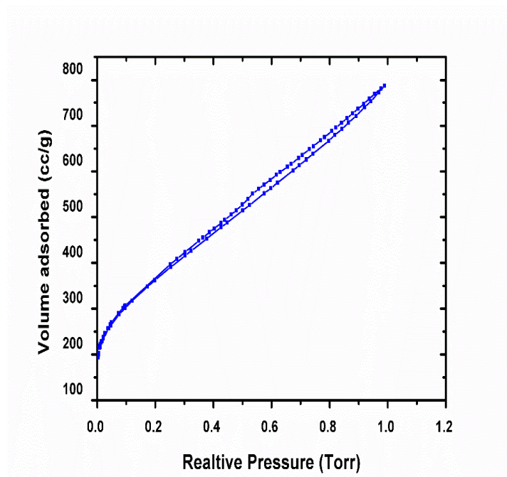
Figure 7: Nitrogen adsorption-desorption isotherms of electrode materials
