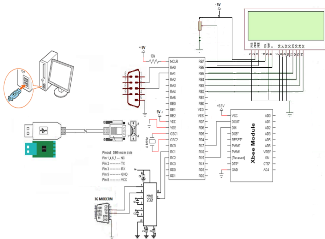
Figure 3: Master unit
