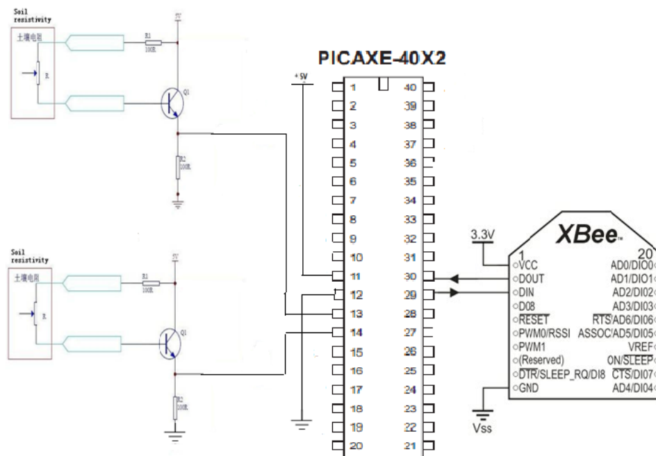
Figure 2: Slave unit
