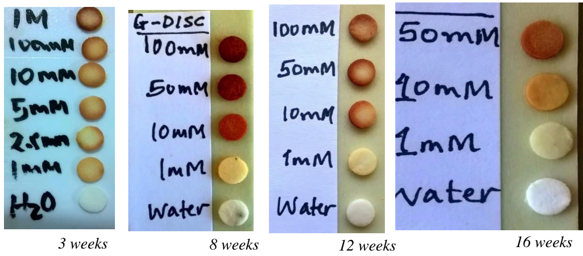
Figure 26. Glucose-disc test using discs stored at ambient conditions for up to 16 weeks
