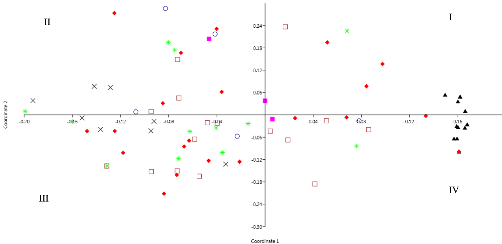
Figure 7: Scatter plot of a PCoA showing the distribution of Corchorus spp. accessions based on ISSR data
