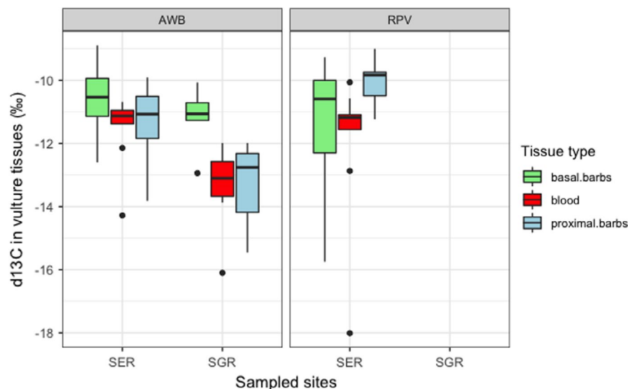
FIGURE 2 \delta^{13}\text{C} ratios in vulture tissues across Serengeti National Park (SER) and Selous Game Reserve (SGR) over time
