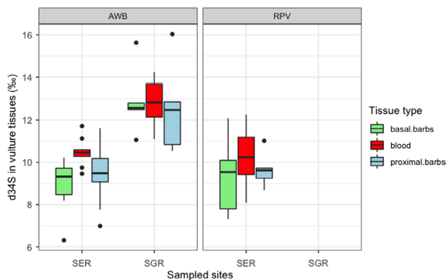
FIGURE 4 \delta^{34}\text{S} ratios in vulture tissues across Serengeti National Park (SER) and Selous Game Reserve (SGR) over time
