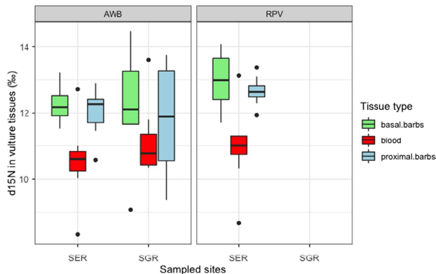
FIGURE 3 \delta^{15}\text{N} ratios in vulture tissues across Serengeti National Park (SER) and Selous Game Reserve (SGR) over time
