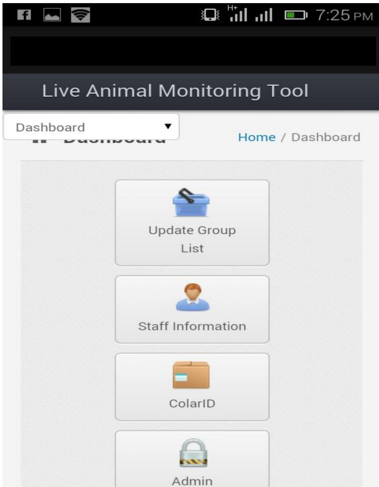
Figure 28: Dashboard
