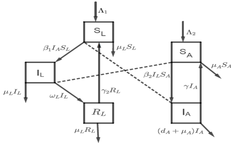
Figure 2: The flow diagram for the spread of Prosopis juliflora plant on piece of land by animals that ingest the plant seeds
