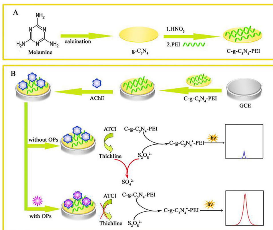
Fig. 5. Schematic description of (A) the preparation process of graphitic carbon nitride-poly (ethylenimine) (C-g-C 3 N 4 -PEI), (B) the fabrication of modified biosensor and response mechanism [115].
