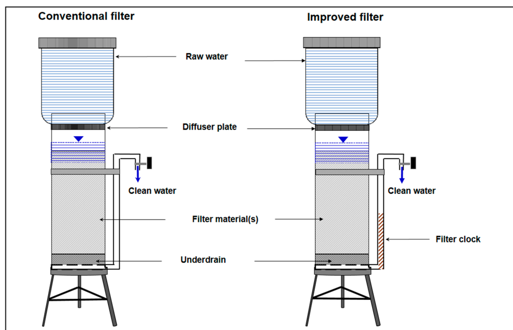
Figure 1. Basic concept of a filter-clock subsequent to a conventional filter. The \text{Fe}^0 -based filter-clock clogs promptly after the exhaustion of the capacity of the conventional filter (at t_\infty ). This operating principle corresponds to the one of colored indicators widely used in Analytical Chemistry (titration reaction).
