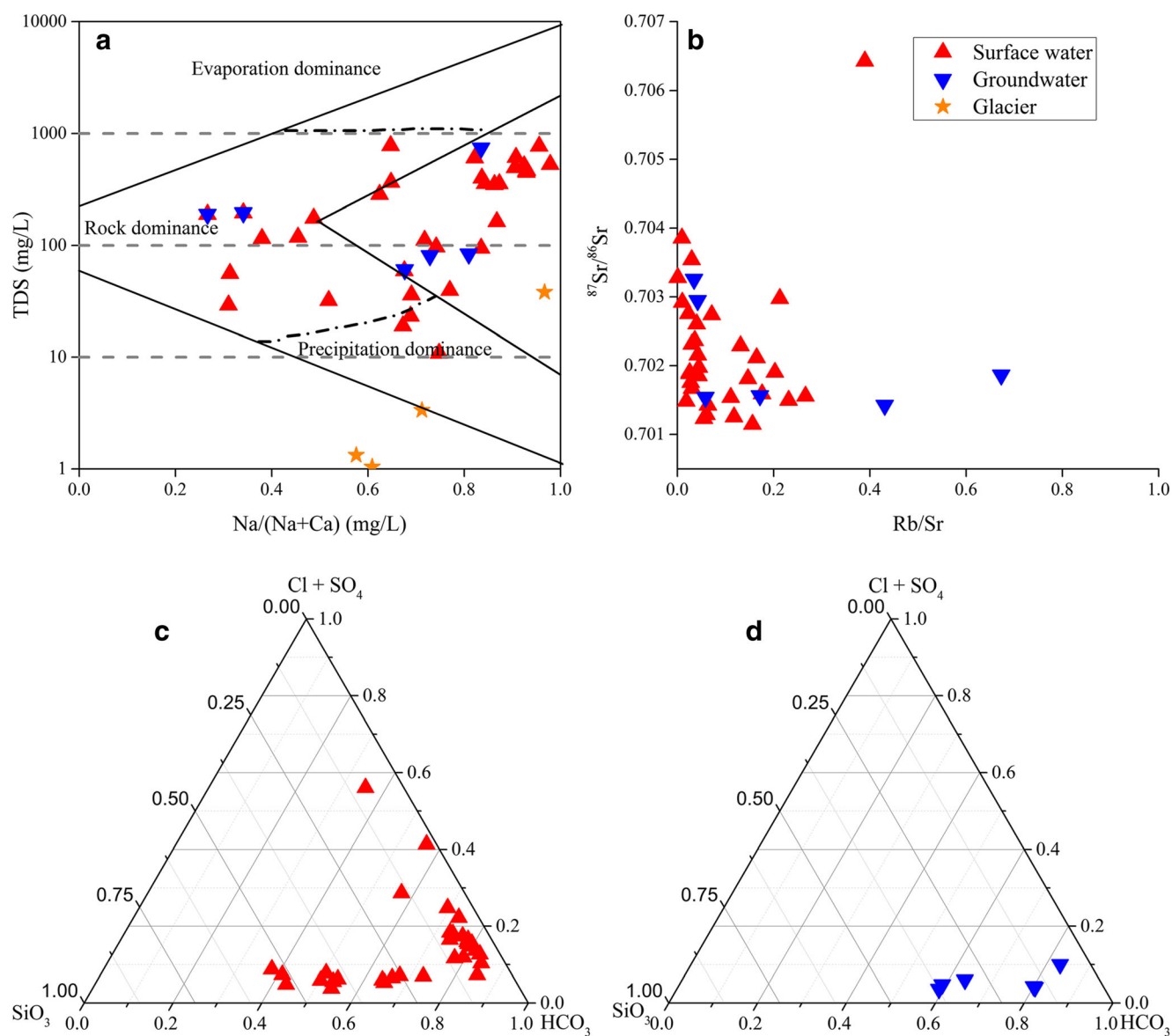
Fig. 5 (a) Major natural process controlling chemistry of PRB. The ratios were adapted from Gibbs (1970). (b) Strontium isotopes and Rb/Sr ratio. (c), (d) are Ternary diagram after atmospheric correction
