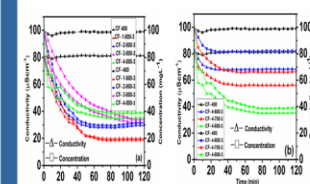
Figure 3: Desalination experiment with the CF carbon electrodes: (a) Impact of KOH: CF ratio; (b) Impact of activation temperature.
