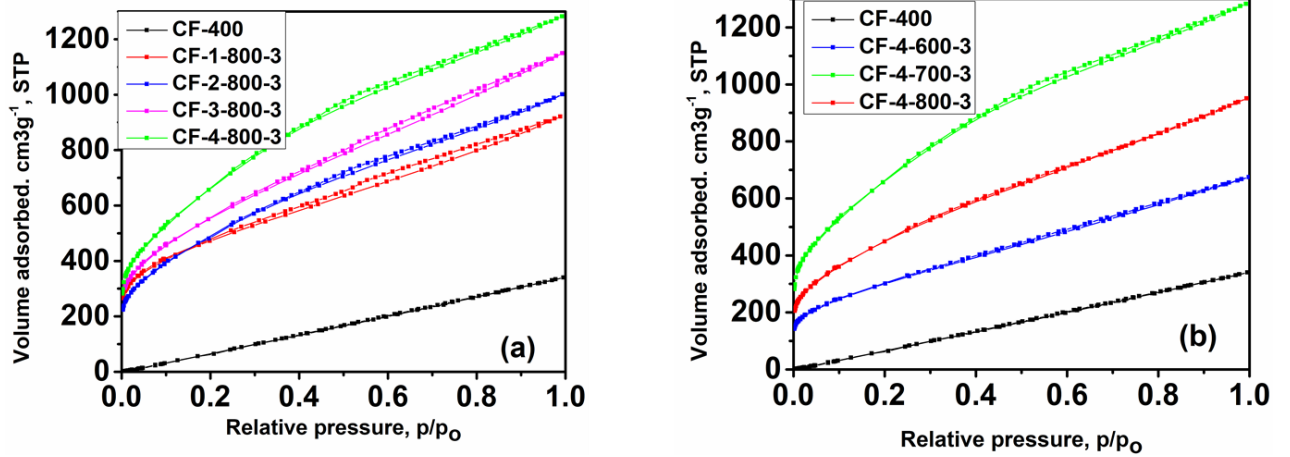
Figure 5: Nitrogen adsorption-desorption isotherms of CF activated carbon samples: (a) Impact of KOH: CF ratio; (b) Impact of activation temperature.
