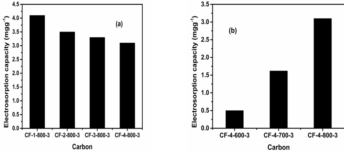
Figure 11: Electrosorption capacity of lead by CF electrodes: (a) Effect of KOH: CF ratio; (b) Effect of activating temperature.
