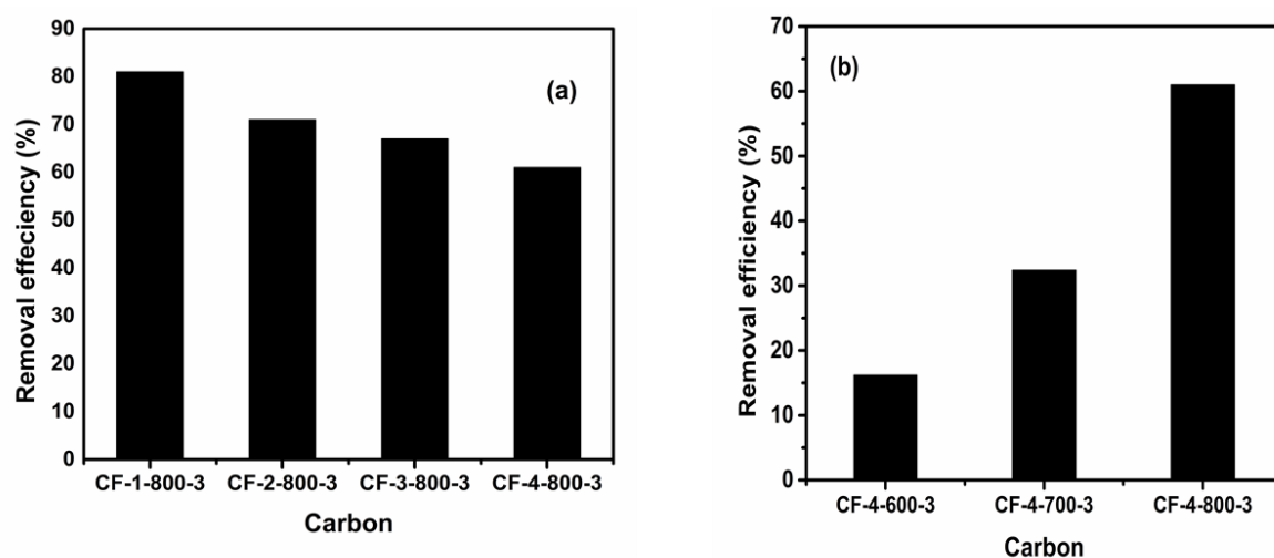
Figure 10: Lead removal efficiency of CF electrodes: (a) Effect of KOH: CF ratio; (b) Effect of activating temperature.
