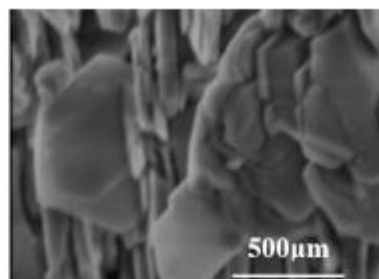
Figure 3. Surface morphology of OLA-TP-850 sample before adsorption.
