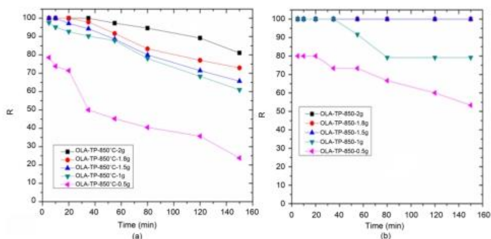
Figure 8. Effect of adsorbent mass on removal efficiency of \text{H}_2\text{S} (a) and \text{NH}_3 (b); OLA-TP-850, flowrate 0.002 \text{ m}^3/\text{min} .
