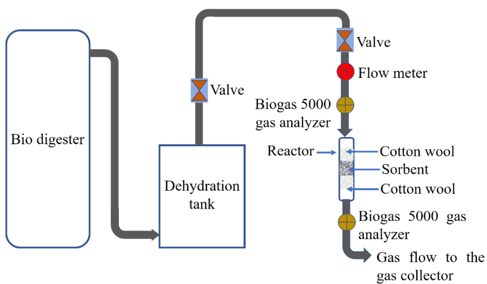
Figure 3: Schematic diagram of the sorption experimental setup.
