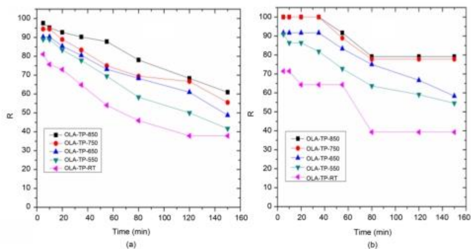
Figure 6. Effect of calcination temperature on removal efficiency of H_2S (a) and NH_3 (b); OLA-TP samples, flowrate 0.002 \text{ m}^3/\text{min} , mass of the adsorbent 1 g.
