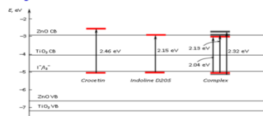
Fig. 6: Energy level diagram of HOMOs and excited state potentials of crocetin, indoline D205 and complex molecules in chloroform.
