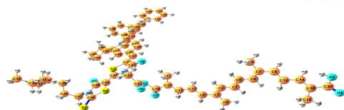
Fig. 3: Optimized geometrical structure of the complex ( C_{68}H_{69}N_3O_7S_3 ).
