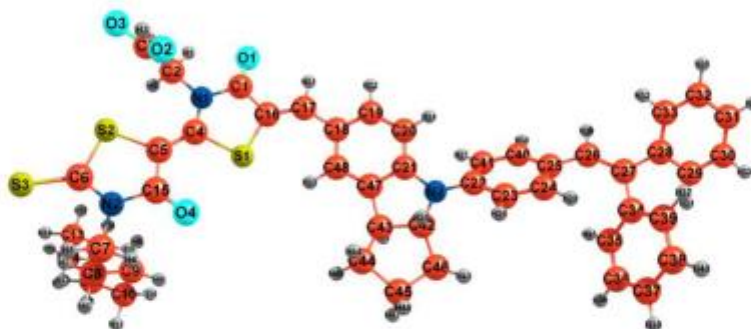
Figure 2. Optimized geometrical structure of the indoline dye D203 molecule.
