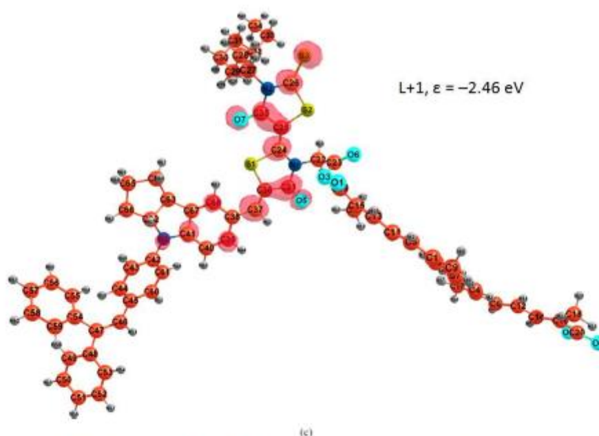
Figure 10. Frontier and adjacent MOs in the complex molecule: (a) HOMO and LUMO; (b) H-1; (c) L+1.
