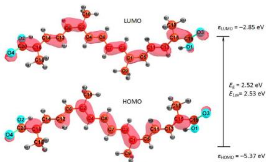
Figure 8. Frontier orbitals HOMO and LUMO in the crocetin molecule.
