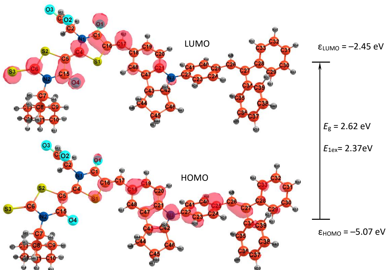
Figure 18: Frontier orbitals HOMO and LUMO in the crocetin molecule.
