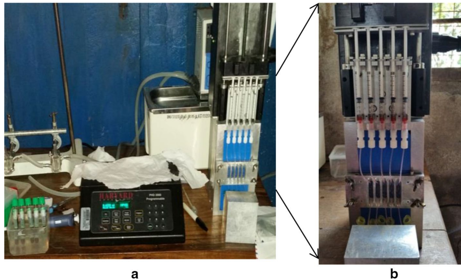
Fig. 2 MDM apparatus used in the field study. a Note five-channel sample flow arrangement operated by a syringe pump and a programmable controller. The flow channel assembly is pressed against the permanent magnet (painted blue) using four wing nuts. b Five blood samples visible inside 1 mL syringes prior to being pumped back into the collection tubes (bottom) through the flow channel pressed against the magnet. The weight of the system is estimated at less than 3 kg
