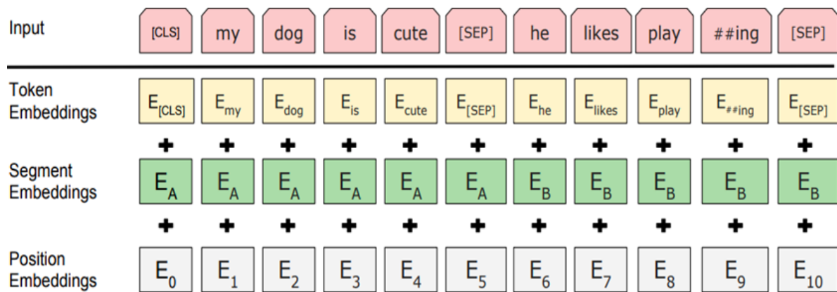
Figure 3: BERT input representation by Devlin et al. (2018)
