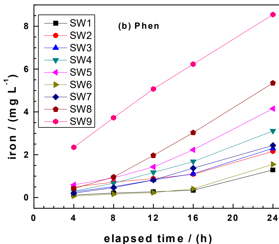
Figure 3. Comparison of the dissolution rate of the tested \text{Fe}^0 SW specimens in (a) ethylenediaminetetraacetic (EDTA) and (b) 1,10 Phenantroline (Phen) under quiescent conditions for 24 h. Experimental conditions: m_{\text{iron}} = 0.10 g, [\text{EDTA}] = [\text{Phen}] = 2 mM, V_{\text{solution}} = 50 mL. The represented lines are not fitting functions; they just connect the points to ease visualization. The regression parameters are listed in Table 2.
