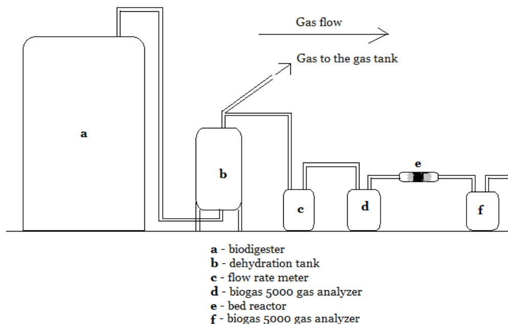
Figure 1. Experimental setup for the \text{H}_2\text{S} and \text{NH}_3 adsorption.
