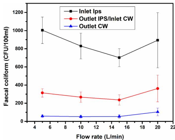
Figure 6 | FC removal by the integrated IPS-CW.
